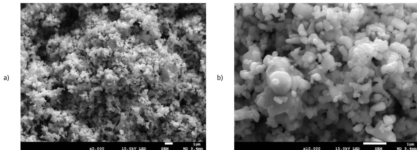
Fig. 1. Scanning electron microscope photos of the POLYDEF Ag+ additive a) 5,000 times magnification, b) 15,000 times magnification
