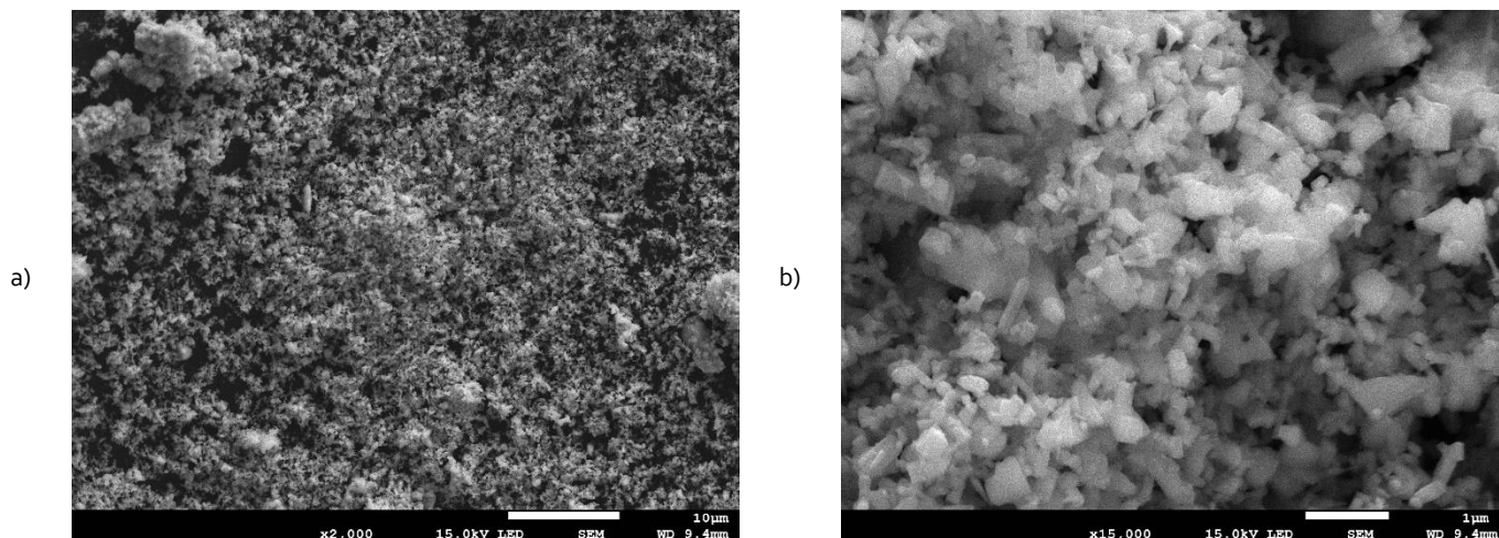
Fig. 1. Scanning electron microscope photos of the POLYDEF Cu+ additive a) 2,000 times magnification, b) 15,000 times magnification
